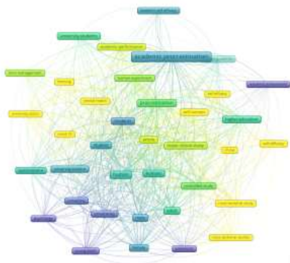
Figure 4. Overlay Visualization
