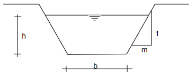
Figure 3. Trapezoidal Channel
